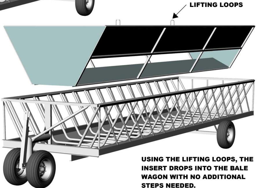
LIFTING LOOPS
